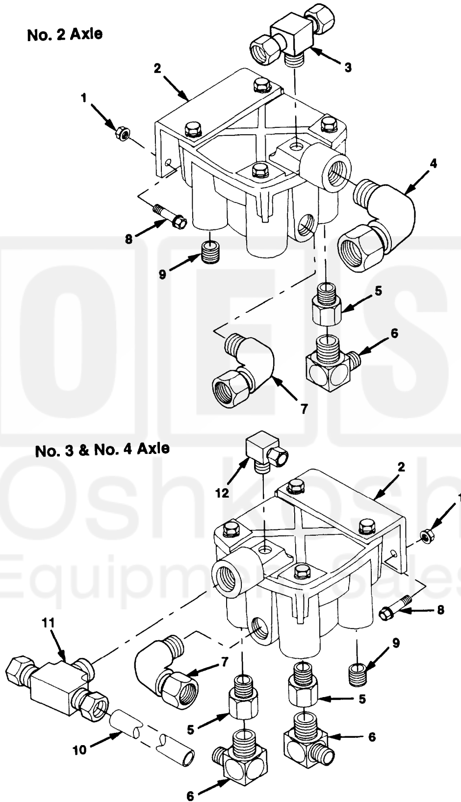
Figure 148. Spring Brake Relay Valves and Fittings
